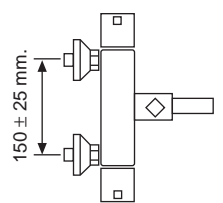
TERMOQUATRO BAÑO-DUCHA TERMOQUATRO BATH-SHOWER
