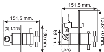
TERMOBASIC BAÑO DUCHA EMPOTRAR TERMOBASIC CONCEALED BATH/SHOWER
