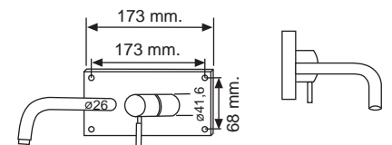
BASIC LAVABO EMPOTRAR BASIC CONCEALED BASIN
